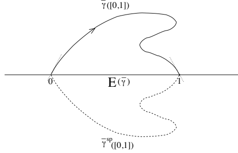
FIGURE 2. An embedded initial datum \bar{\gamma} , with its specular one (dotted curve) and the region E(\bar{\gamma}) enclosed between the two curves. The points (0, 0) and (1, 0) are the two triple junctions, if one imagines to add to the curves the horizontal half lines on the left of (0, 0) and on the right of (1, 0) .
