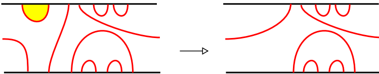
Figure 6.14. Two homotopic simple closed curves in a torus are isotopic: put them in transverse position, cut the first to get an annulus, then remove bigons to destroy intersections.
