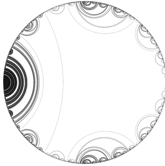
Figure 8.4. A geodesic lamination in \mathbb{H}^2 .
