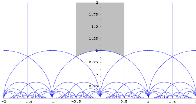
Figure 3.15. The shadowed triangle (with one ideal vertex) is a fundamental domain for \Gamma = \mathbb{P}\mathrm{SL}_2(\mathbb{Z}) acting on the half-space H^2 . The translates of the fundamental domain form the tessellation shown.
