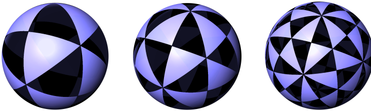
Figure 3.5. The tessellations (2, 3, 3) , (2, 3, 4) and (2, 3, 5) of the sphere.
