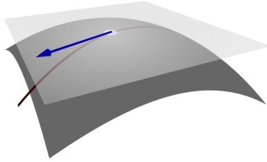
Figure 1.2. The tangent space at p is defined as the set of all curves \gamma with \gamma(0) = p seen up to an equivalent relation that identifies two curves having (in some chart) the same tangent vector at p . This is a chart-independent condition.
