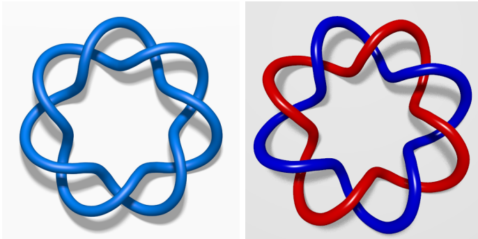
Figure 11.7. The torus knot (2, -7) and the torus link (2, -8) .
