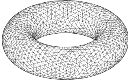
Figure 1.7. A triangulated torus.
