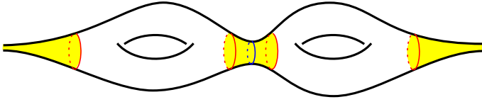
Figure 4.3. The thick-thin decomposition of a complete hyperbolic surface: the thin part (yellow) consists of truncated cusps and neighbourhoods of short geodesics (blue).
