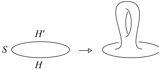
Figure 11.1. A stabilisation of a Heegaard splitting.
