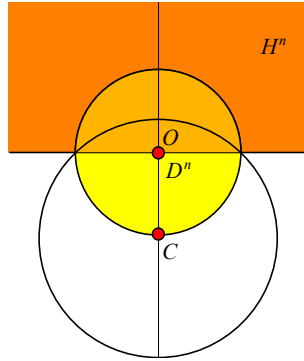
Figure 2.6. The inversion along the sphere with centre C = (0, \dots, 0, -1) and radius \sqrt{2} transforms the Poincaré disc D^n into the half-space model H^n . Here n = 2 .
