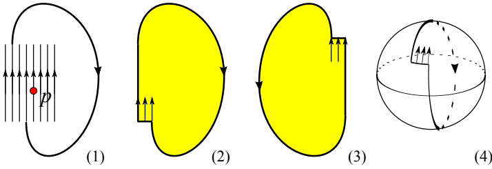
Figure 6.23. At a point p , after a local diffeomorphism we may suppose that the vector field is constantly vertical (1). If p is a limit point of an integral curve \alpha we may find a closed curve that bounds a disc (2). If such a disc existed, we could rotate it and inverse all arrows (3) and glue the two portions to form a nowhere-vanishing vector field on the sphere (4).
