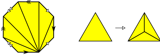
Figure 7.14. The standard representation of S_g by identifying the edges of a 4g -gon has one vertex; we triangulate the 4g -gon and get an ideal triangulation for S_{g,0,1} (left). A move that modifies a triangulation by adding a new vertex (right).
