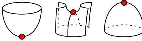
Figure 9.1. Non-degenerate points of index 0, 1, and 2.
