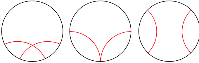
Figure 2.11. Two incident, asymptotic parallel, and ultra-parallel lines.
