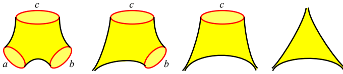
Figure 6.5. A pair-of-pants, an annulus with one puncture, a disc with two punctures, and a thrice-punctured sphere. The last three surfaces may be considered as some degenerated hyperbolic pairs-of-pants where one or more boundary lengths a , b , or c are zero, and we get cusps instead of geodesic boundary components there.
