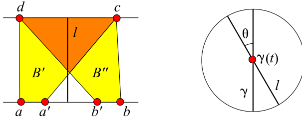
Figure 8.2. The box B containing l and the sub-boxes B' , B'' (left). A line l \in U_\gamma parametrised as (t, \theta) (right).
