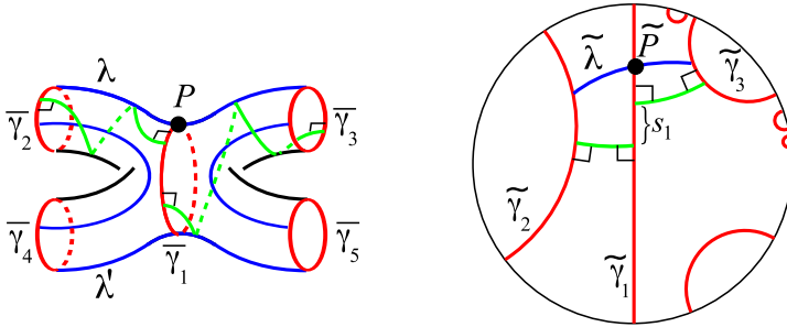
Figure 7.9. A closed geodesic \bar{\gamma}_1 and the two adjacent pairs-of-pants. The torsion parameter \theta_1 measures the distance (in the universal covering) between two orthogeodesics (coloured in green) via the formula \theta_i = \frac{2\pi s_i}{l_i} .
