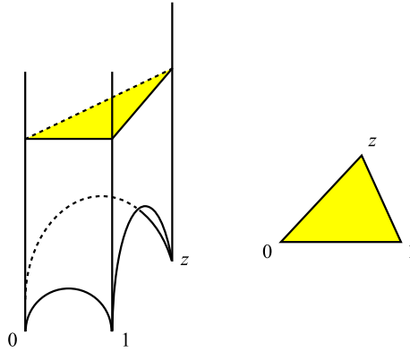
Figure 14.1. An ideal tetrahedron with three vertices in 0, 1, \infty in the half-space mode is determined by the position z \in \mathbb{C} \cup \{\infty\} of the fourth vertex. A small horosphere centred at the ideal vertex intersects the tetrahedron in a Euclidean triangle uniquely determined up to similarities.
