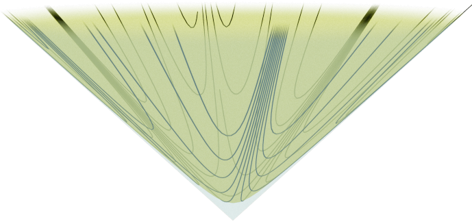
Figure 5.3. The \Gamma -invariant decomposition of the hyperbolic plane into ideal polygons obtained by projecting the Euclidean polygons of Figure 5.2 from \partial C to I^2 . This is in fact the Farey tessellation of Figure 5.1.
