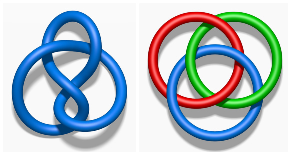
Figure 14.9. The figure-eight knot and the Borromean rings are hyperbolic , that is their complements admit complete hyperbolic metrics.
