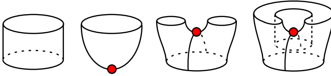
Figure 9.4. After capping off at each u_i we end up with many spheres of these basic types, which clearly bound balls.
