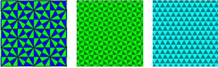
Figure 3.6. The tessellations (2, 3, 6) , (2, 4, 4) , and (3, 3, 3) of the Euclidean plane.
