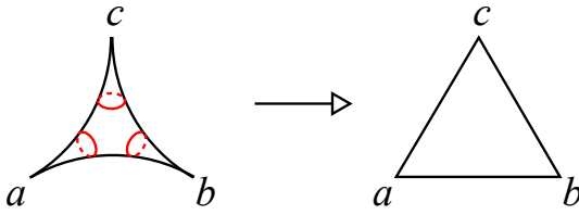
Figure 3.20. The index-two orientation-preserving \Gamma^{or}(a, b, c) \triangleleft \Gamma(a, b, c) defines an index-two orbifold covering O \rightarrow \Delta , where O is a 2-sphere with three singular points and \Delta a triangle.
