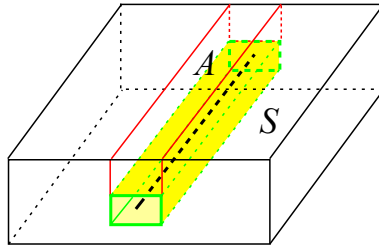
Figure 11.12. We push \gamma in a collar for \partial H_2 and drill a solid torus neighbourhood, drawn here as a yellow parallelepiped.
