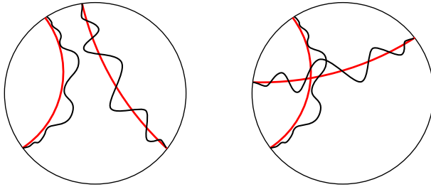
Figure 6.17. The lifts of \gamma (black arcs) and of its geodesic representative (red lines) have the same endpoints in \partial\mathbb{H}^2 (left). If two lines intersect, the arcs do (right).
