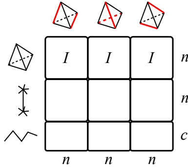
Figure 15.12. The enlarged matrix \bar{A} .
