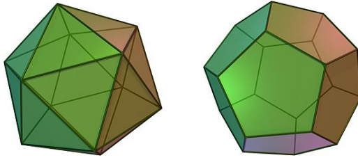
Figure 3.3. The regular icosahedron and dodecahedron.
