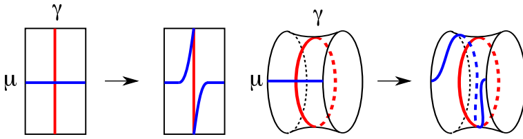
Figure 6.26. A Dehn twist along a curve \gamma maps a transverse arc \mu onto an arc which makes a complete left turn.
