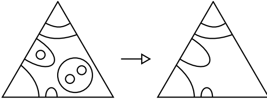
Figure 9.11. The closed curves contained in a triangle are the intersections of small spherical components of S with that triangle. We just remove them.
