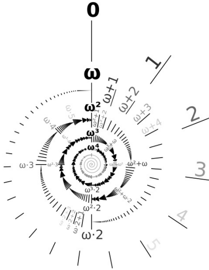
Figure 15.14. The volumes of complete orientable hyperbolic 3-manifolds form a well-ordered subset of \mathbb{R} of type \omega^\omega .
