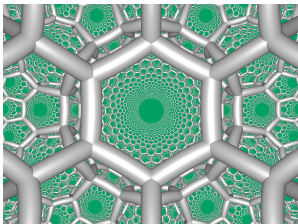
Figure 3.13. In the tessellation \{6, 3, 3\} of \mathbb{H}^3 every polyhedron has infinitely many hexagonal faces, whose vertices all lie in a single horosphere.
