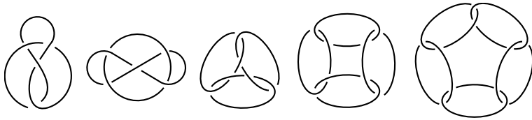
Figure 14.10. A remarkable sequence of hyperbolic links. These are the figure eight knot , the Whitehead link , and some particular chain links with 3,4,5 components.
