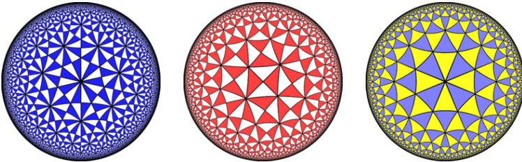
Figure 3.7. The tessellations (2, 3, 7) , (2, 4, 5) , and (3, 3, 4) of the hyperbolic plane.
