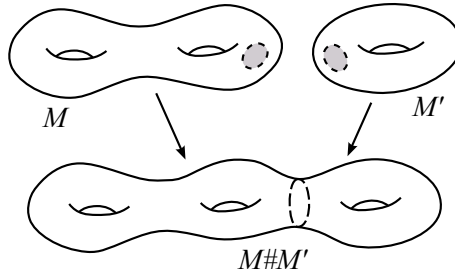
Figure 1.3. A connected sum of closed surfaces.
