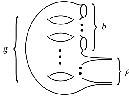
Figure 6.4. The finite type surface S_{g,b,p} .
