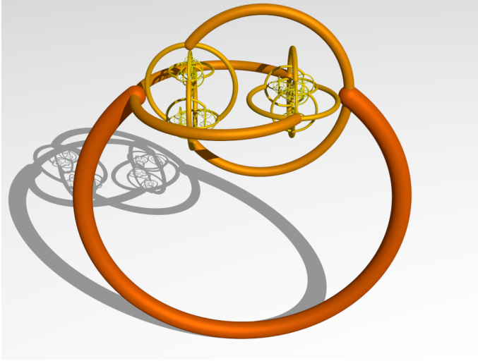
Figure 1.1. The Alexander horned sphere is a subset of \mathbb{R}^3 homeomorphic to the 2-sphere S^2 . It divides \mathbb{R}^3 into two connected components, none of which is homeomorphic to an open ball. It was constructed by Alexander as a counterexample to a natural three-dimensional generalisation of Jordan's curve theorem. The natural generalisation would be the following: does every 2-sphere in \mathbb{R}^3 bound a ball? If the 2-sphere is only topological, the answer is negative as this counterexample shows. If the sphere is a differentiable submanifold, the answer is however positive as proved by Alexander himself.
