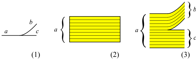
Figure 8.11. How to construct a lamination from a weighted train track. Here we have a switch with weights a, b, c (1) and the switch condition a = b + c allows all the Euclidean rectangles (2) to glue (3).
