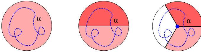
Figure 9.24. The immersed curve \alpha intersects k \leq 3 regions and is hence of one of these types (because B is essential).
