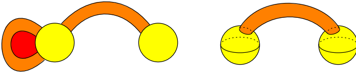
Figure 1.6. Two 0-handles (yellow), two 1-handles (orange), one 2-handle (red) in dimension 2 (left). Two 0-handles (yellow), a 1-handle (orange) in dimension 3 (right).
