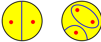
Figure 10.14. Essential vertical annuli and tori in a Seifert manifold fibering over a disc with 2 or 3 singular points.
