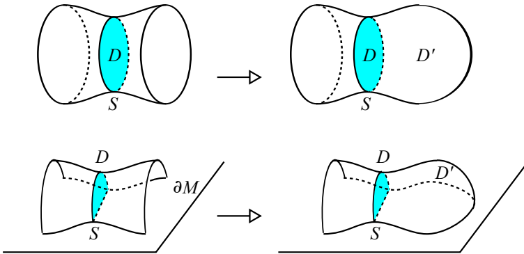
Figure 9.16. A surface S is incompressible ( \partial -incompressible) if the existence of a disc D as in the top-left (bottom-left) picture implies the existence of another disc D' \subset S as in the top-right (bottom-right) picture. If in addition M is irreducible ( \partial -irreducible) the two discs D and D' form a sphere (disc) which bounds a ball (is \partial -parallel), and hence by substituting D' with D we get two isotopic surfaces.
