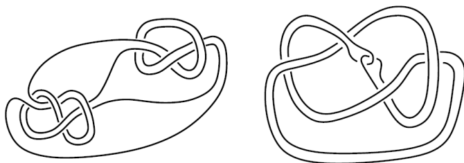
Figure 11.9. Two satellite knots.
