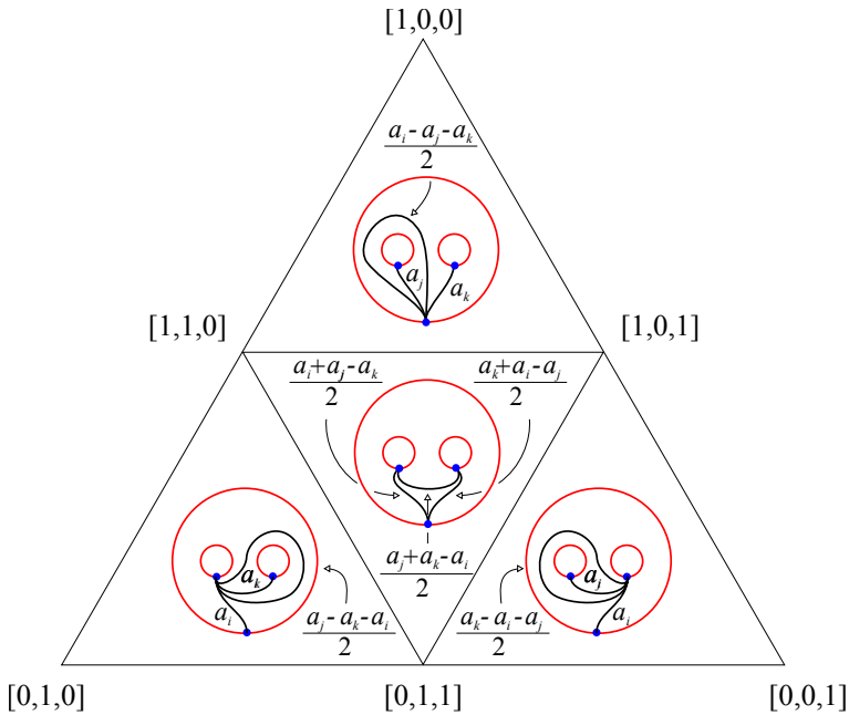
Figure 8.9. The portion of weighted train track in a pair of pants P is determined by the point Q = [a_i, a_j, a_k] \in \mathbb{RP}^2 . Having non-negative entries, the point Q is contained in the triangle with vertices [1, 0, 0] , [0, 1, 0] , [0, 0, 1] . This triangle subdivides into four sub-triangles by adding the vertices [0, 1, 1] , [1, 0, 1] , [1, 1, 0] and the shape of the train track depends on which sub-triangle contains Q . The three edges of the train track are given the weights indicated in the figure: these are the only weights that sum to a_i, a_j, a_k at the boundaries. When Q lies in the frontier of two or more triangles some branch has weight zero and we delete it: the different shapes prescribed by the adjacent triangles coincide after deleting this branch.
