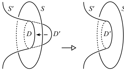
Figure 9.15. The discs D and D' form a sphere which bounds a ball since M is irreducible. We can use this ball to isotope S' away from S .
