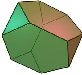
Figure 14.3. A truncated tetrahedron.
