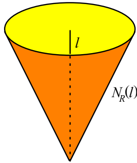
Figure 4.1. The R -neighbourhood N_R(l) of a vertical line in the half-space model is a Euclidean cone. The boundary of the cone is not totally geodesic: the cone is however convex.
