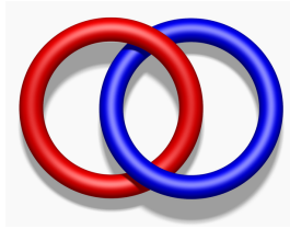
Figure 11.8. The Hopf link is the (2, 2) -torus link.
