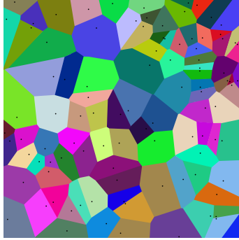
Figure 3.14. A Voronoi tessellation of the Euclidean plane.
