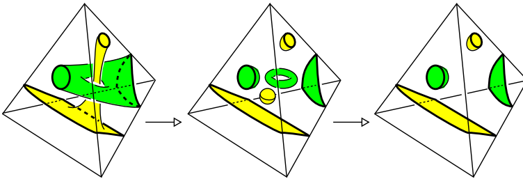
Figure 9.10. Starting from the innermost curves in \partial\Delta \cap S we surger along discs so that S \cap \Delta consists only of discs and closed components, which we then remove.
