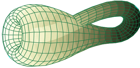
Figure 6.10. The Klein bottle immersed in \mathbb{R}^3 .
