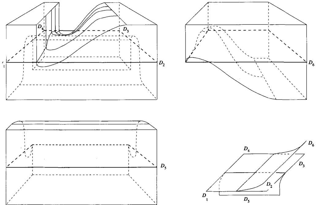
Fig. 11. - Smooth embedding in three dimensions.
