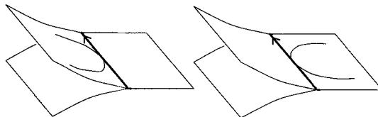
Fig. 1. – Simple tangencies of index +1 and -1 respectively.
