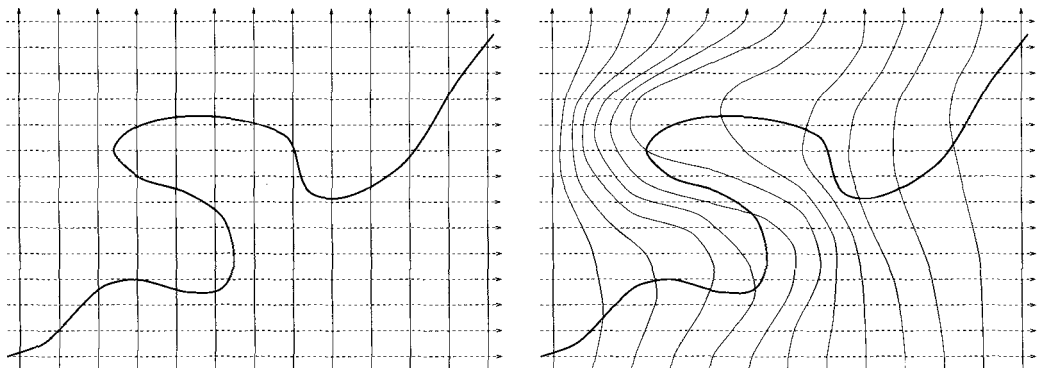
Fig. 8. – Modification of the flow.
