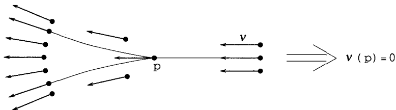
Fig. 4. - A vanishing result for vector fields.
