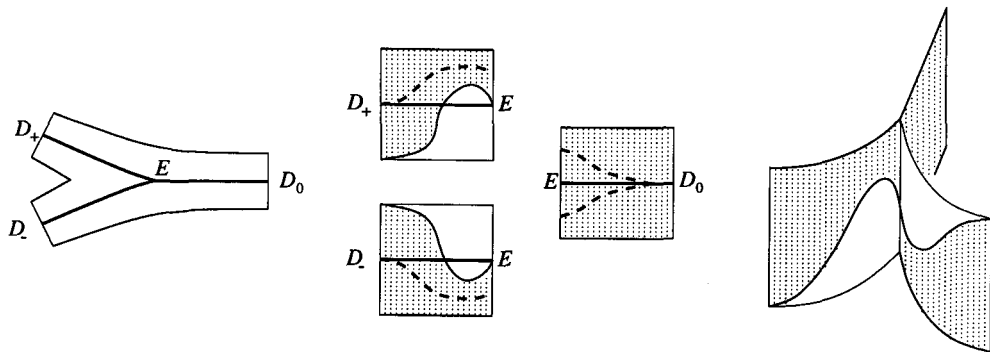
Fig. 10. - Smooth embedding in two dimensions.
