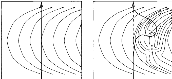
Fig. 9. – How to remove a tangency of index -1 .
