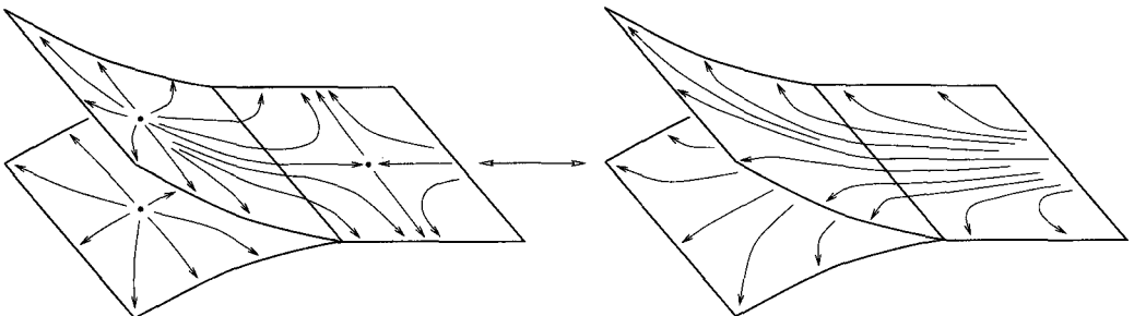
Fig. 6. - Branched elimination lemma II.
