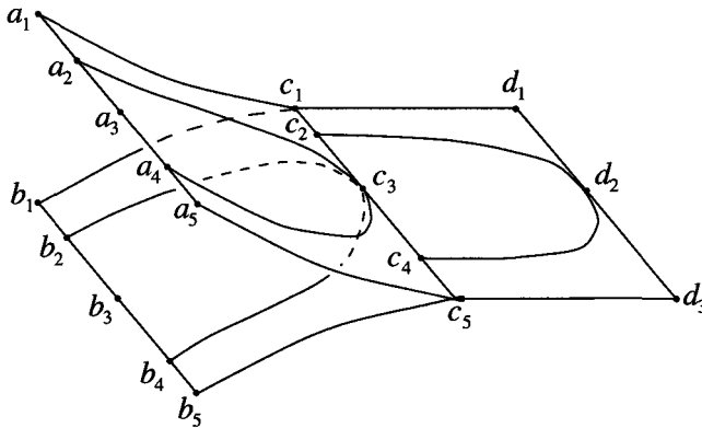
Fig. 3. - Local aspect of a singularity of index +1.
