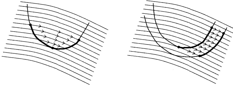
Fig. 2. - Functions defined following the leaves.
